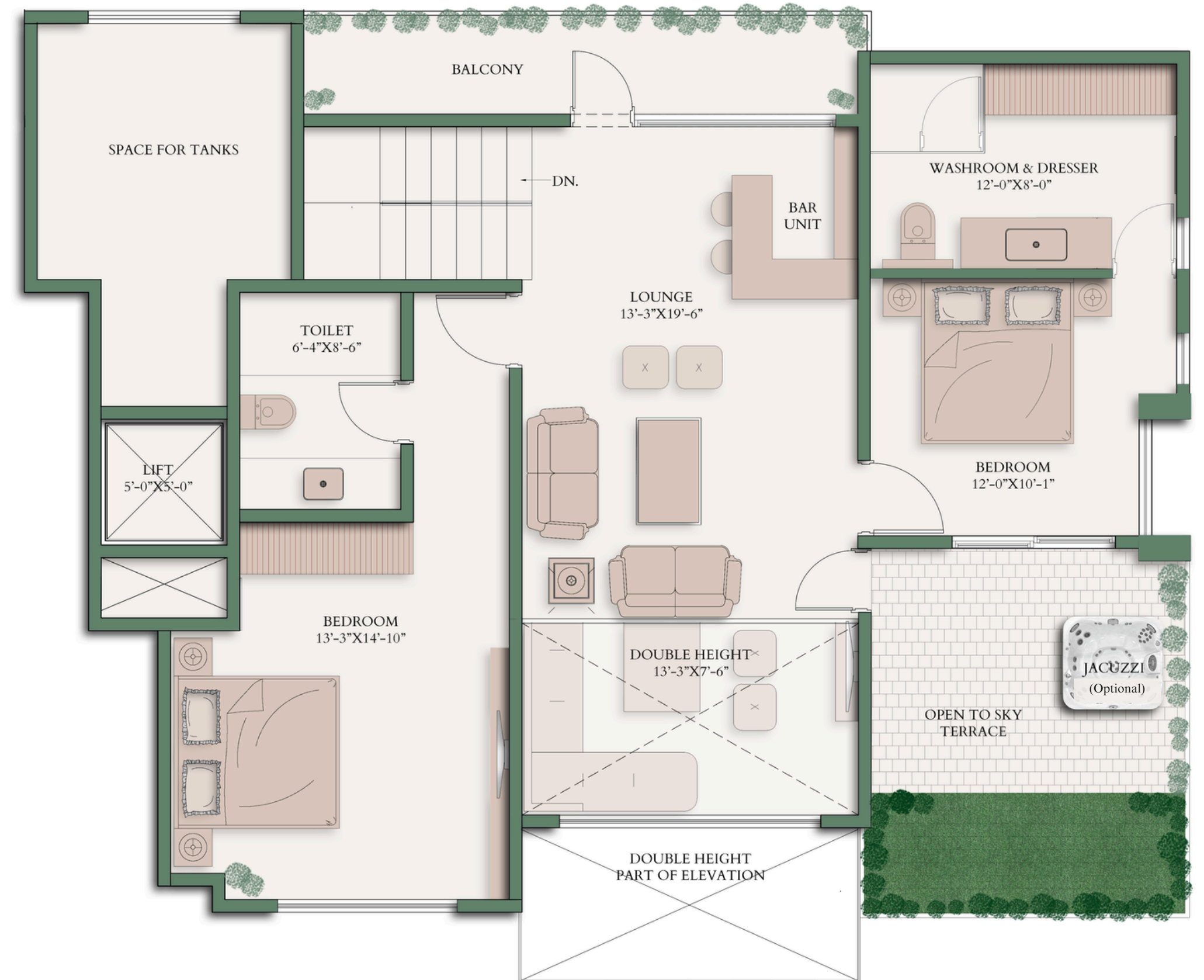
Upper Floor
